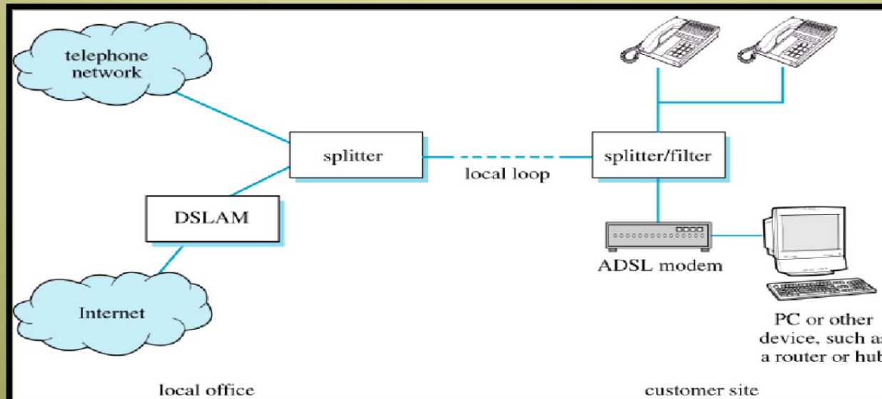
Asymmetric DSL (ADSL) Connection
