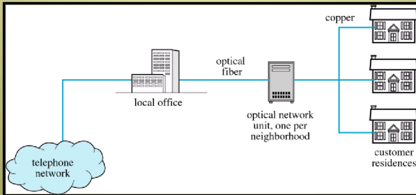
Local Loop: Fiber/Copper Hybrid
