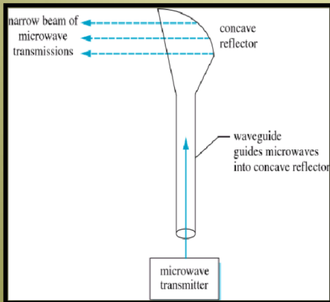
Horn Antenna
