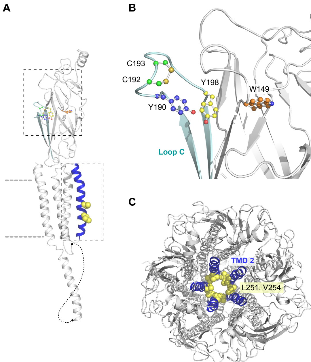
Figure 3: (A) Structure of the acetylcholine receptor \alpha -subunit with functionally relevant structures (cyan: Loop C; blue: pore-lining TMD 2) and residues highlighted. Note also that the 66 amino acids missing in the cytoplasmic domain are depicted as a dotted line. Boxes denote the functionally important regions expanded in panels B and C. (B) Close up view of the \alpha -subunit side of the ligand-binding site, with side chains of residues known to be important for binding shown in ball and stick representations. (C) View of the entire acetylcholine receptor pentamer where the second transmembrane domain (TMD 2) of each subunit has been coloured blue. Van der Waals spheres of hydrophobic residues that form the ion channel gate are shown in yellow.
