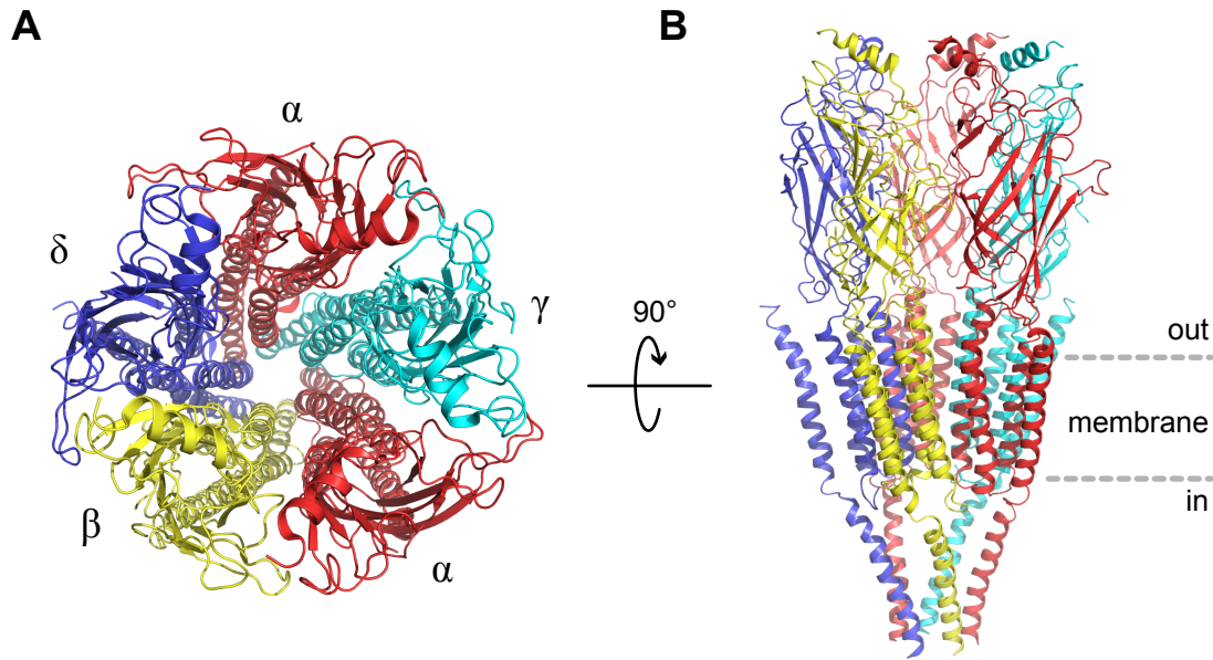
Figure 1: (A) Overall architecture of the nicotinic acetylcholine receptor from Torpedo mar- morata (PDB ID: 2BG9). View is looking down the central pore axis. Note the pseudosymmet- ric pentameric assembly is composed of 5 homologous subunits ((2 \alpha ) \gamma\delta\beta ). (B) Side view showing the limits of the membrane.
