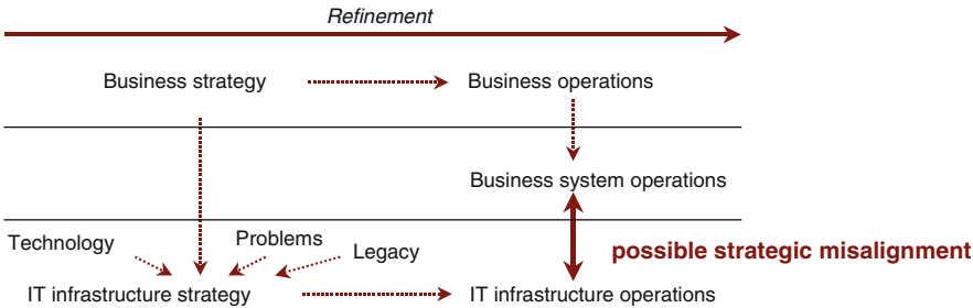
Fig. 9.11 Strategic misalignment
