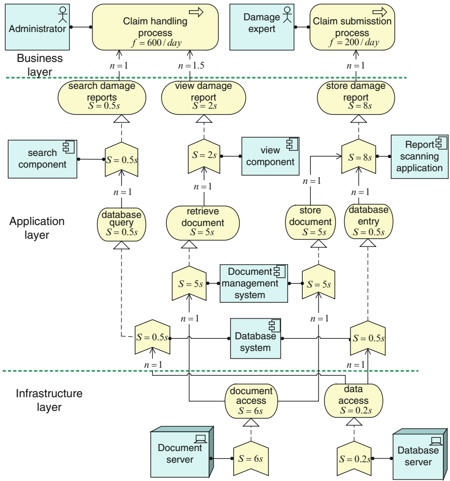
Fig. 8.7 Normalised model
