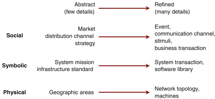
Fig. 9.5 Refinement relations
