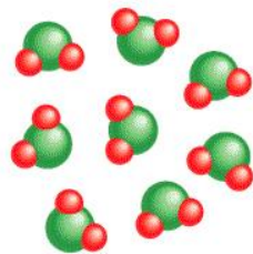
Compound of elements X and Y
