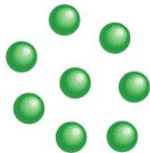
Atoms of element Y
