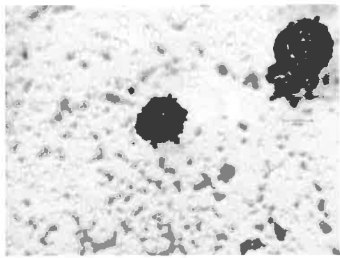
Photo 4: Oil Soot (x40). Dark, translucent cenospheres.
