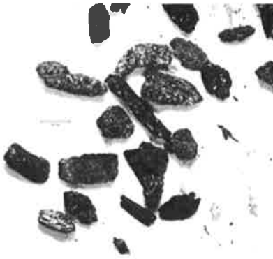
Photo 11: Wood Char (x16). Carbonized, opaque, black, shiny on the surface.
