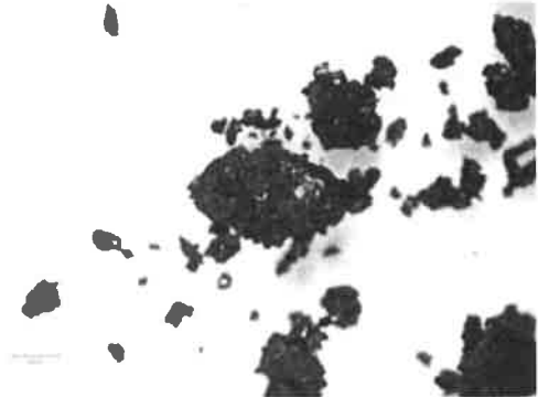
Photo 2: Coal (x16). Black, opaque, sharply angular.
