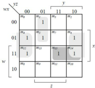
(a) F = xz' + w'y'z + wxy
