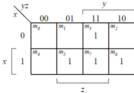
(a) F(x, y, z) = \Sigma(3, 5, 6, 7)
