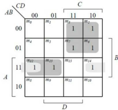
(b) F = A'C + ABC' + ABD'
