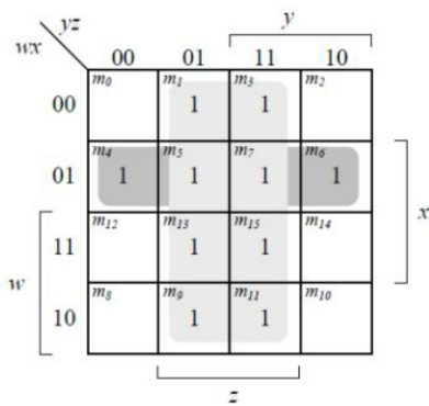
(c) F = z + xw'
