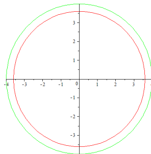
Figure 2: Level curves: R = \sqrt{13} , R = 4
