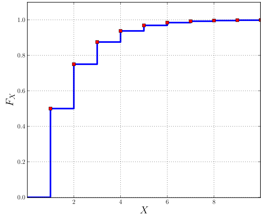
Probability distribution function F_X .
