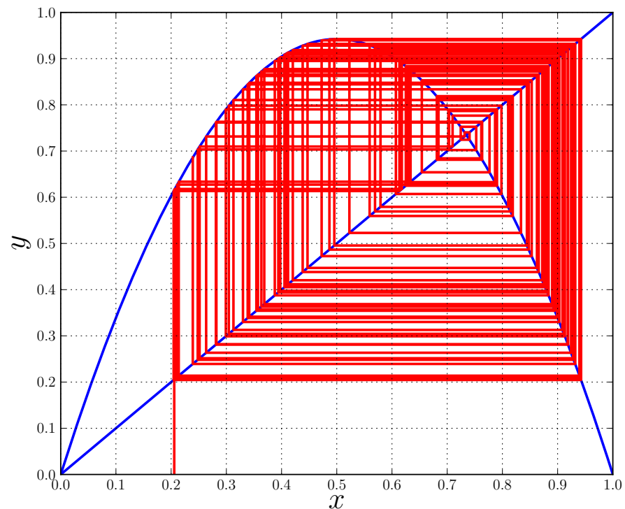
Graphical interpretation.
