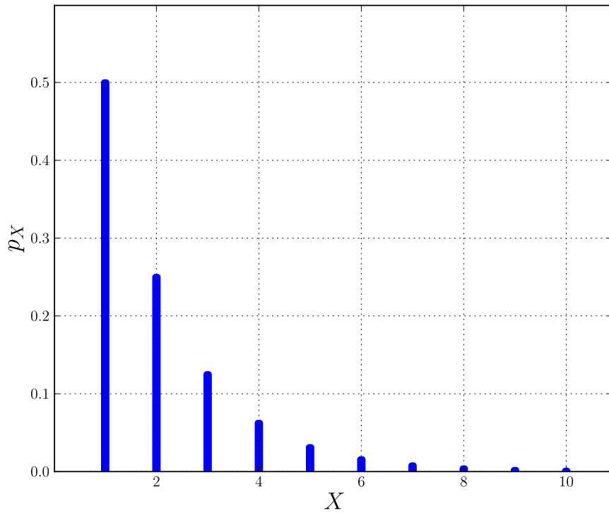
Probability mass function p_X .
