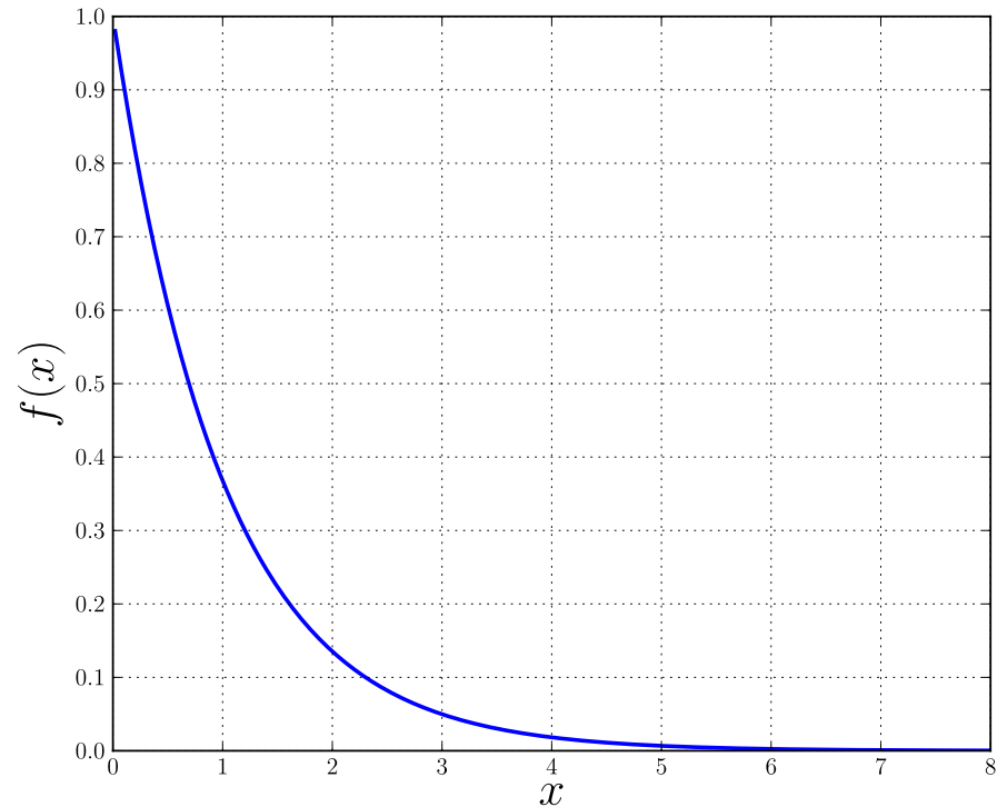
Density function
