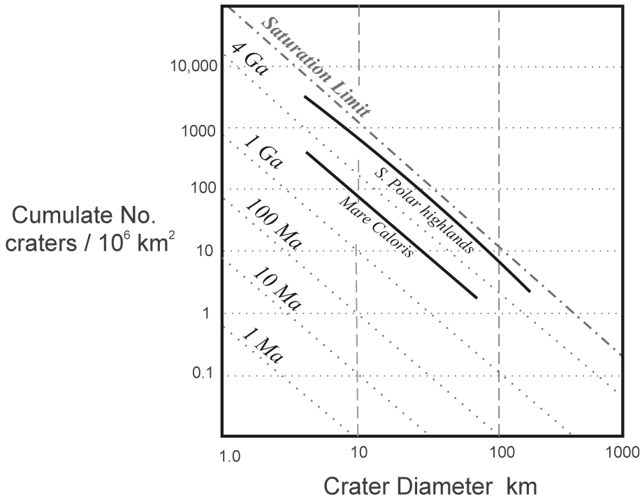
The age of Mercury's surface
