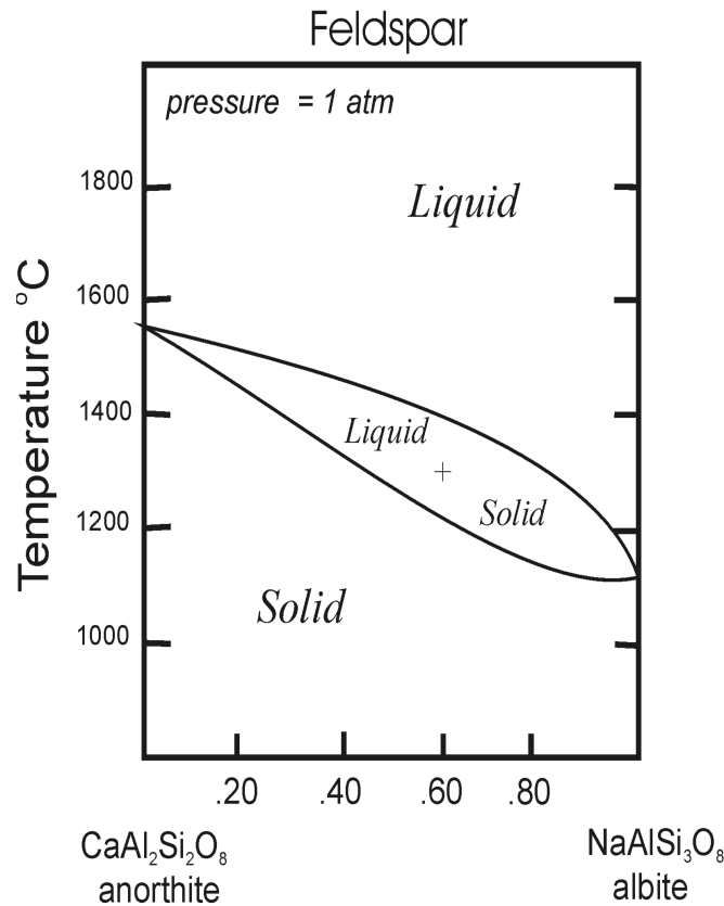
A simple phase diagram for the mineral feldspar.
