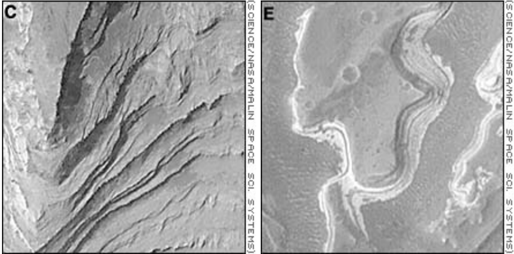
High resolution images of Mars' surface showing possible beaches and shorelines of ancient lakes and oceans (From NASA [free-for-use copyright], Malin SSS)
