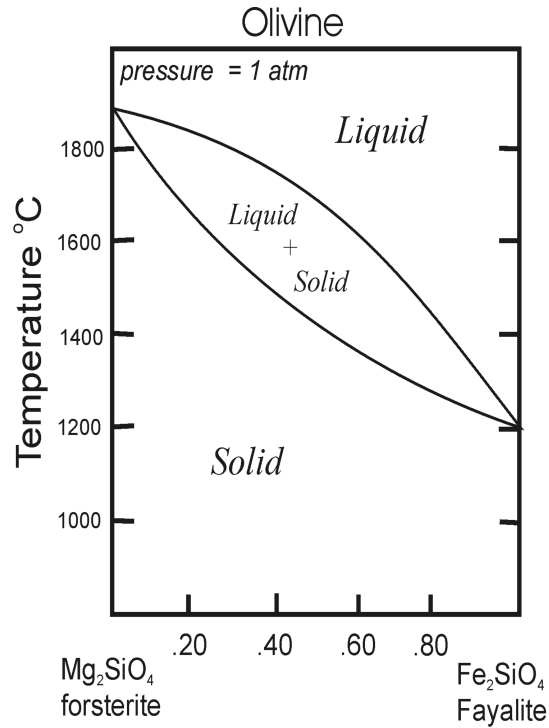
A simple phase diagram for the [\text{Mg,Fe}]_2\text{SiO}_4 olivine.
