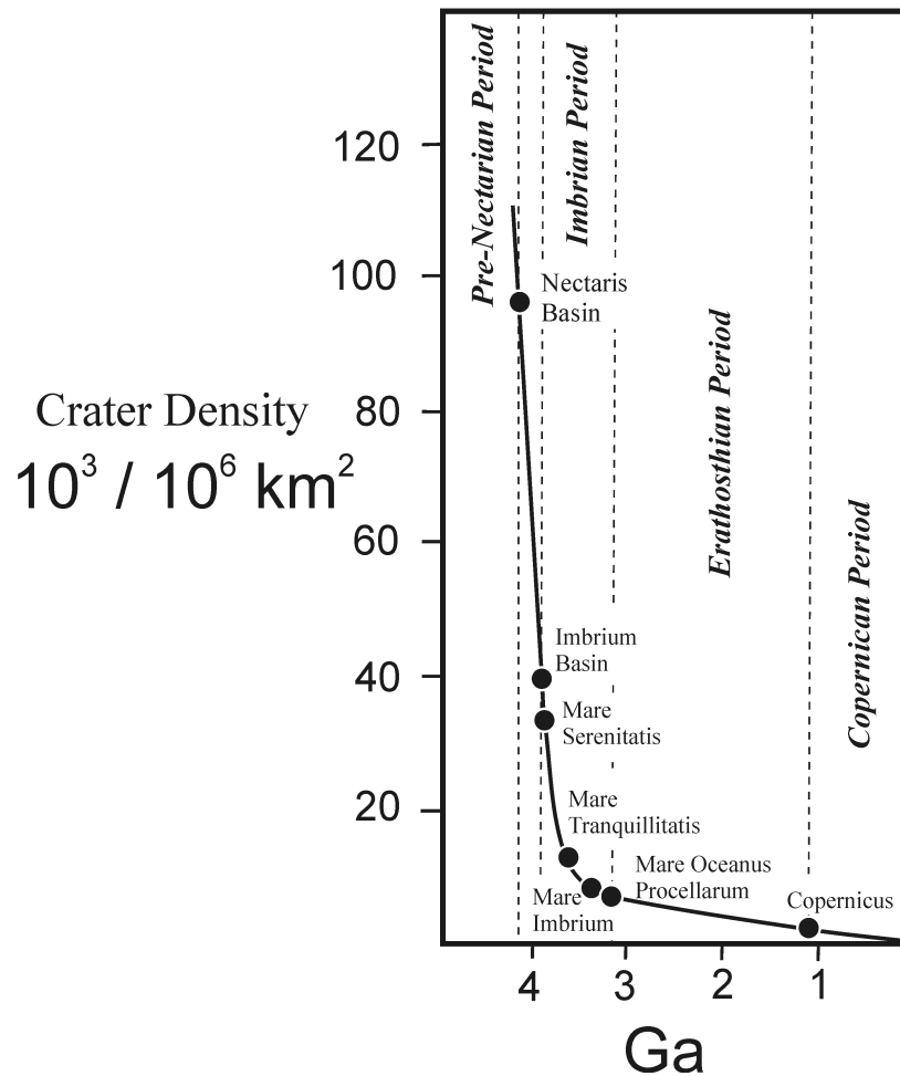
Lunar cratering and age of the Moon's surface features (after D. Francis, Earth & Planetary Sciences, McGill )
