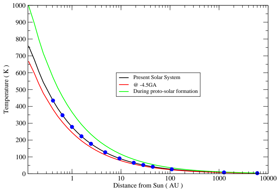
Black-body Temperature in Solar System
