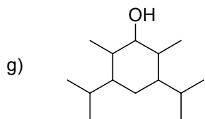
2,6-dimethyl-3,5-diisopropylcyclohexanol
