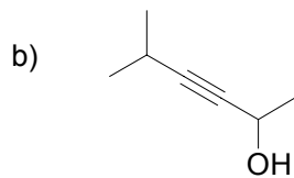
5-methylhex-3-yn-2-ol
