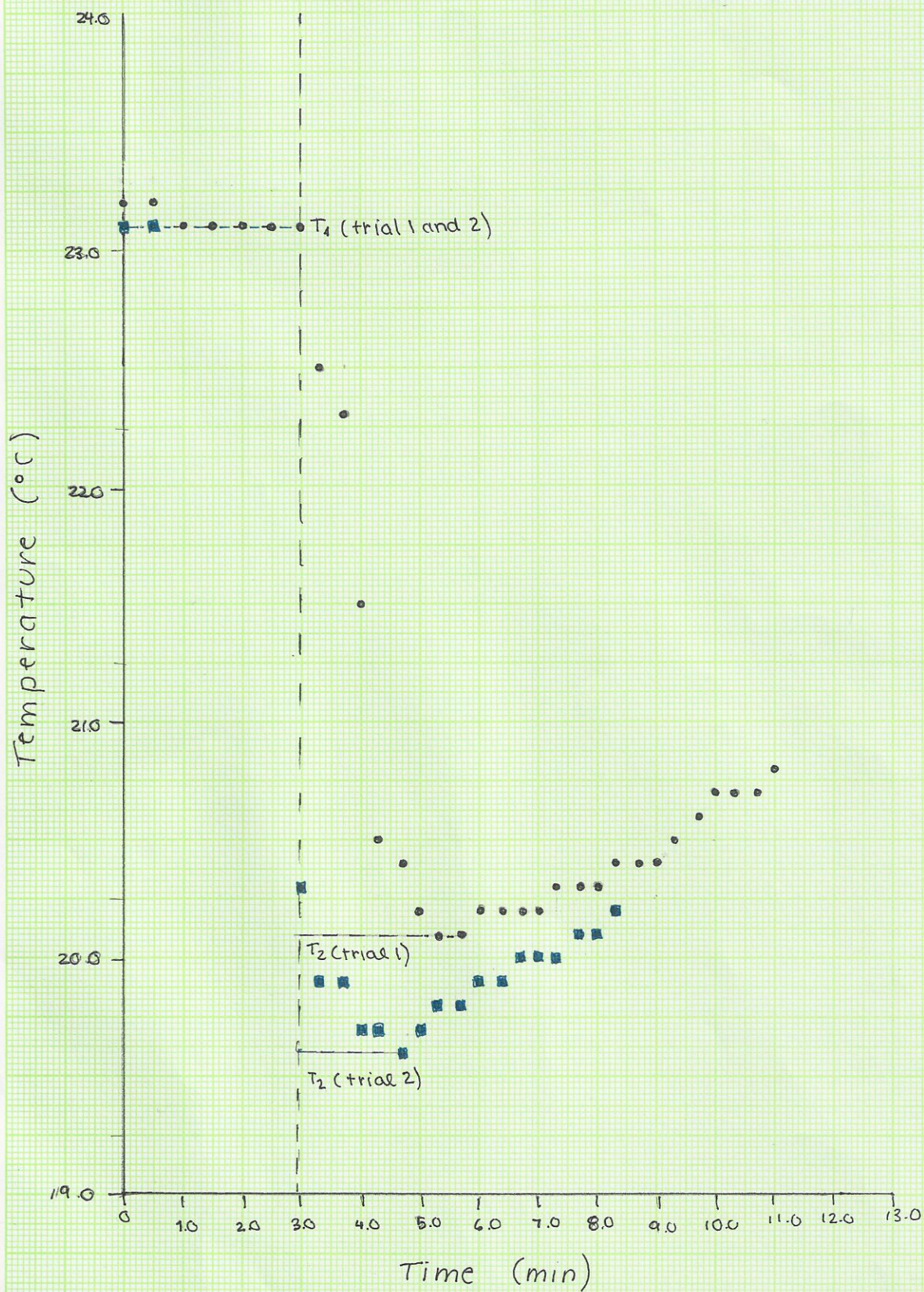
Figure 4: Determining the enthalpy of dissolution using SALT C and observing a change in temperature over time
