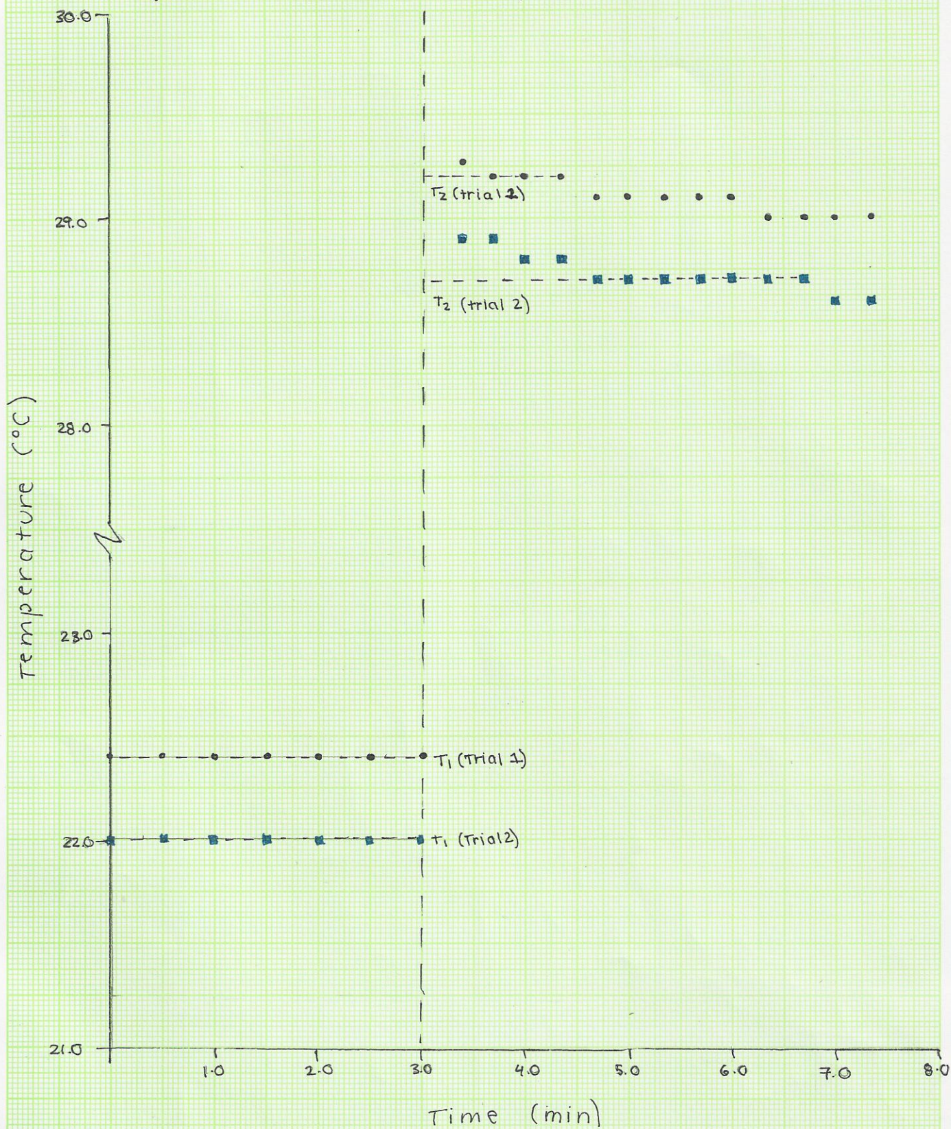
Figure 3: Determining the enthalpy of neutralization using \text{HNO}_3 and observing a change in temperature over time
