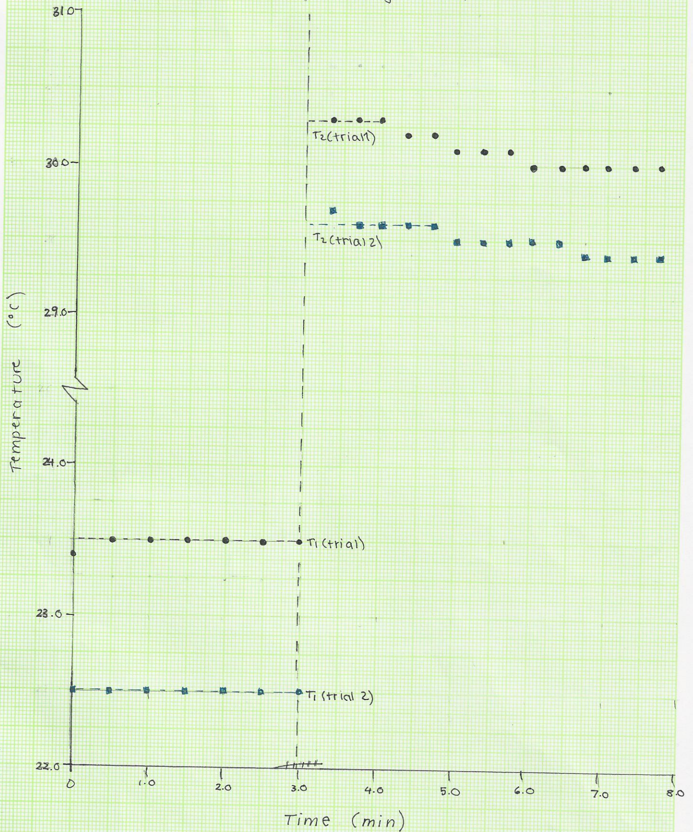
Figure 2: Determining the enthalpy of neutralization using HCl and observing a change in temperature over time
