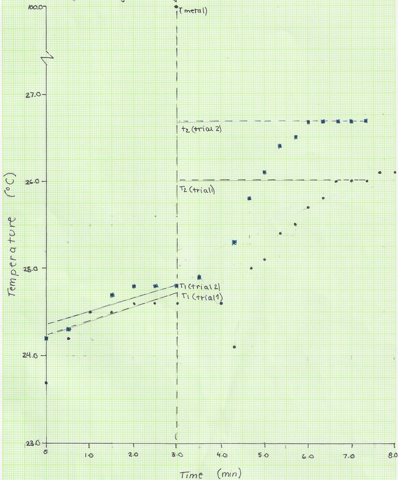
Figure 1: Determining the enthalpy of zinc by observing a change in temperature over time
