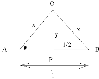
An RT45 Isosceles Triangle
