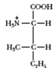
L-Isoleucine (2S,3S)-Isoleucine
