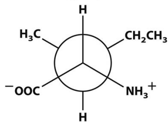
(2S,3S)-Isoleucine
