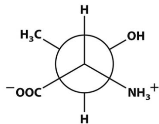
(2S,3R)-Threonine
